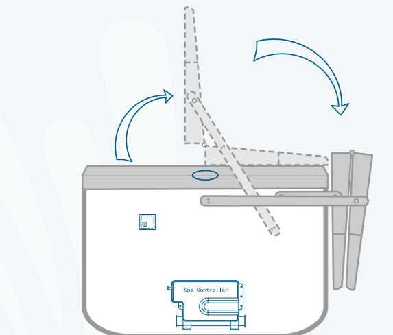
Right-mounted opening
