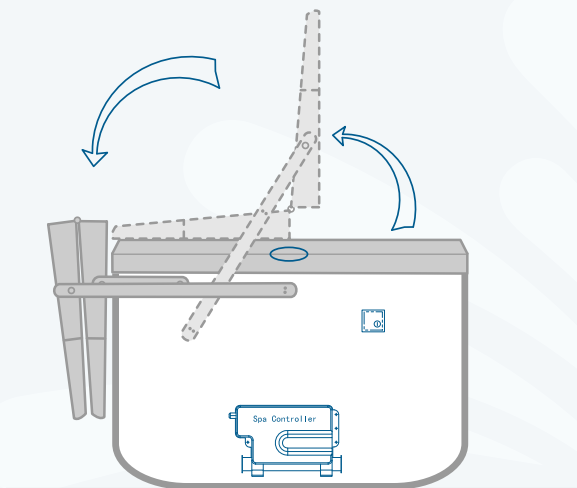
Left-mounted opening
